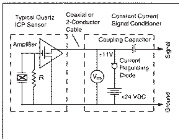
Figure 1.1 ICP® Sensor System Schematic
